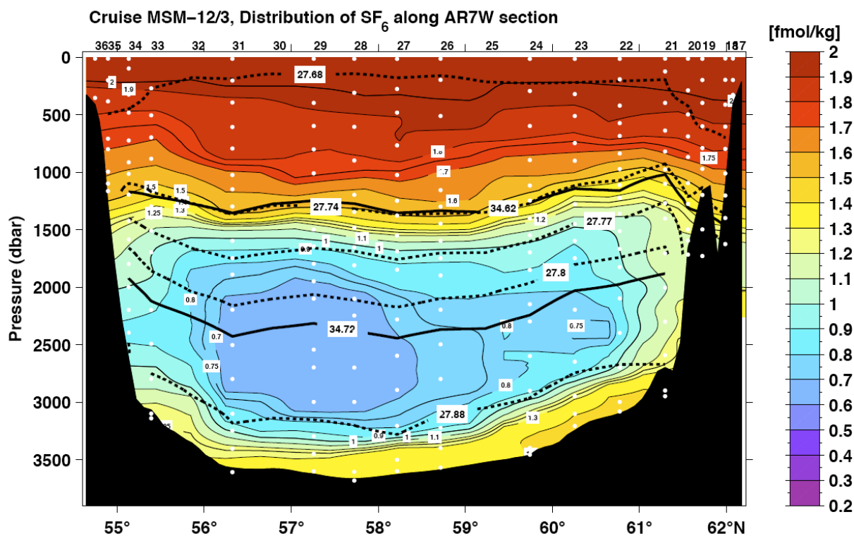
Fig. 5.4 SF 6 section across the Labrador Sea. The contrast between the tracer-poor deeper and denser Labrador Sea Water modes (bound by isopycnals \sigma_{\theta} 27.74 and 27.80) and the SF 6 -rich upper LSW modes (bound by isopycnals \sigma_{\theta} 27.68 and 27.74) is clearly visible. The maximum at the bottom characterizes Denmark Strait Overflow Water (DSOW), \sigma_{\theta} > 27.88 ). Preliminary data
