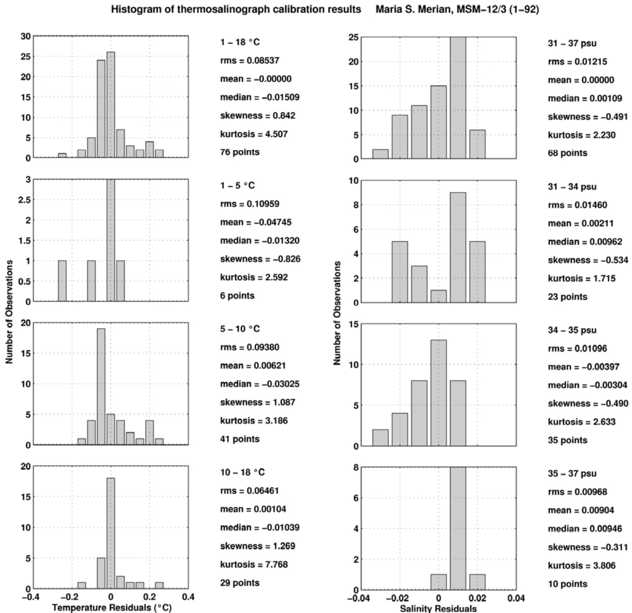
Fig. 5.8 Calibration of the thermosalinograph, MSM 12/3. Right column: temperature, left column: salinity.
